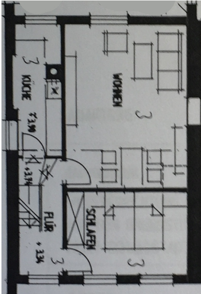
Grundriss 1OG
